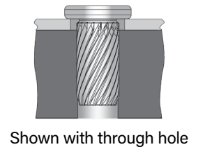
AFTER PRESSING
