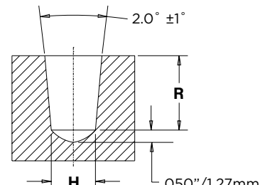
Tapered Hole
